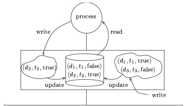
Fig. 7. Basic concepts of the semantics.
