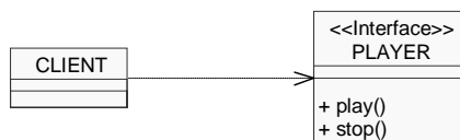
Figure 4: UML model of a media player
