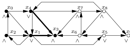
Fig. 5. Computation of c and s by SOLVE
