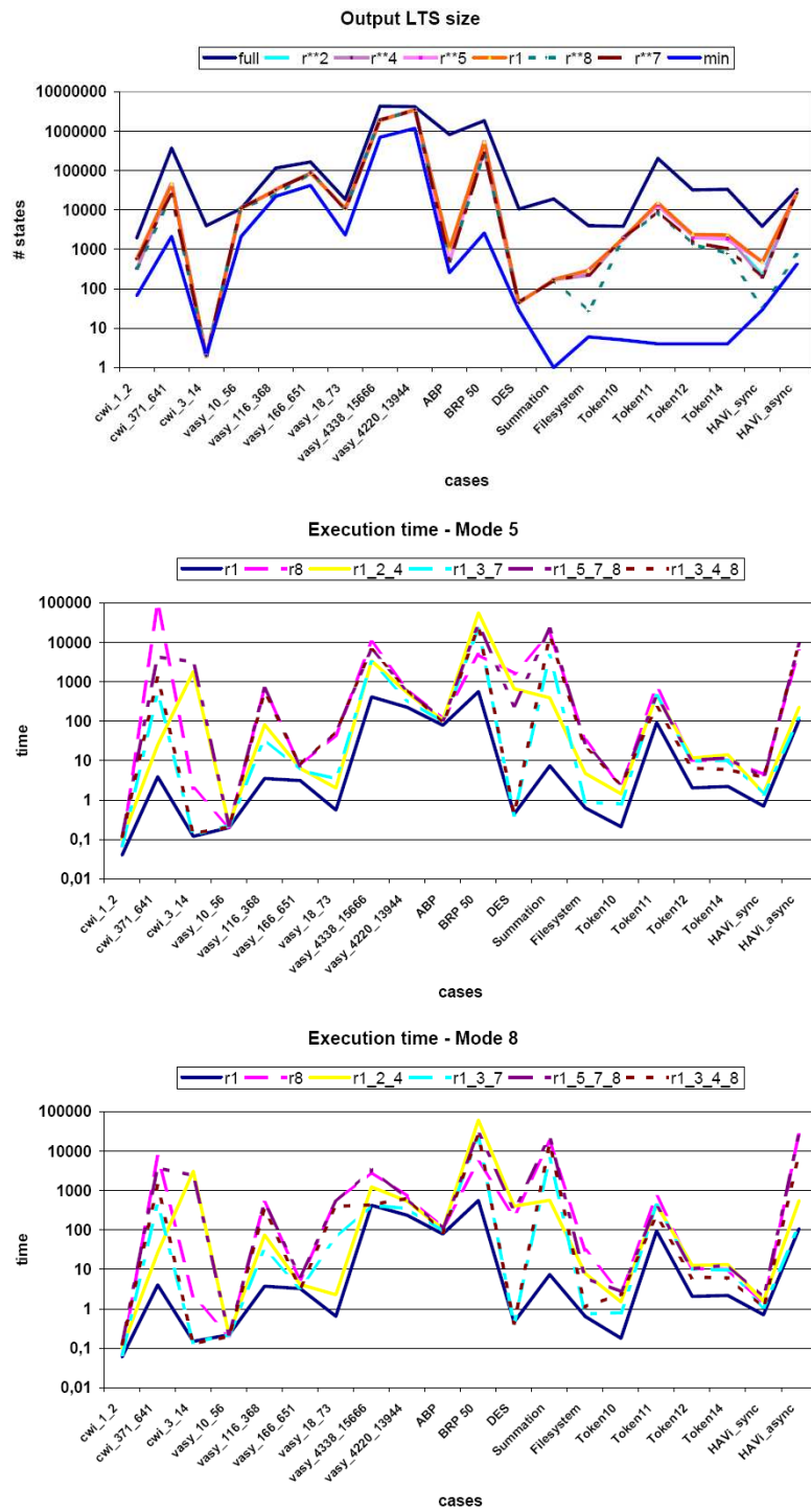
Figure 3: Performance of weak \tau -confluence reductions (I)
